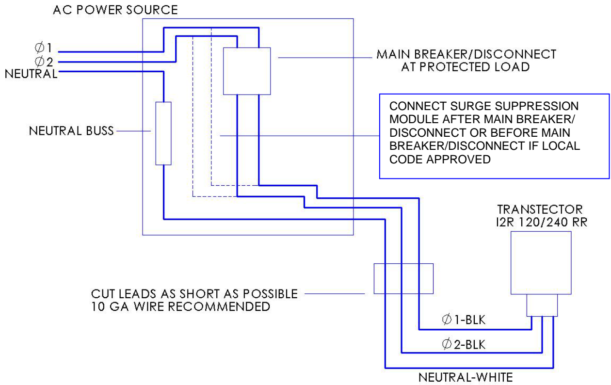
Figure 4: Wiring Diagram
