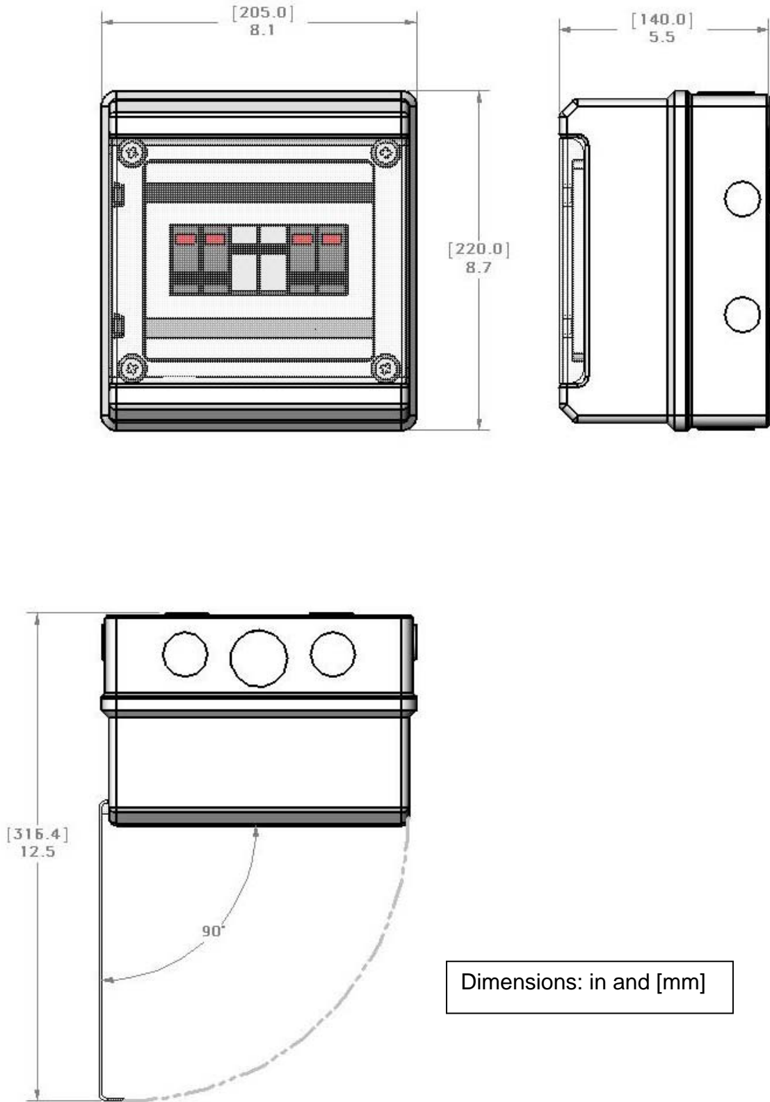
Figure 1: Mechanical Outline
