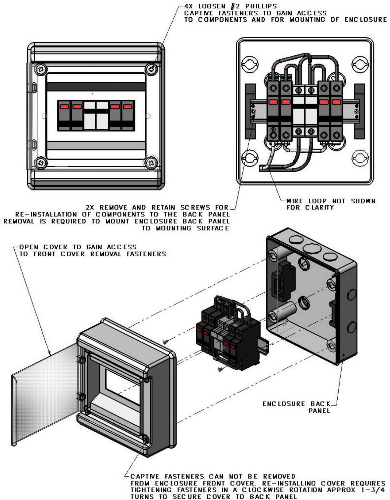
Figure 2: Disassembly for Installation
