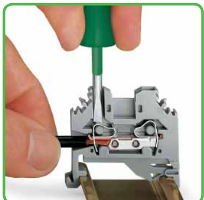
Side-entry wiring: CAGE CLAMP® connection
